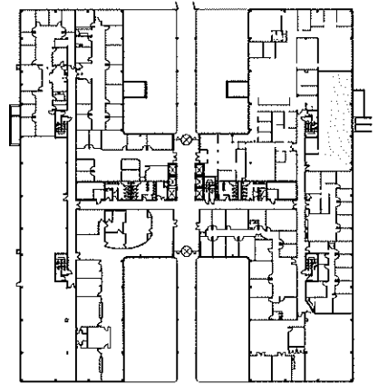
① FIRST FLOOR SUITE 112 FLOOR PLAN
